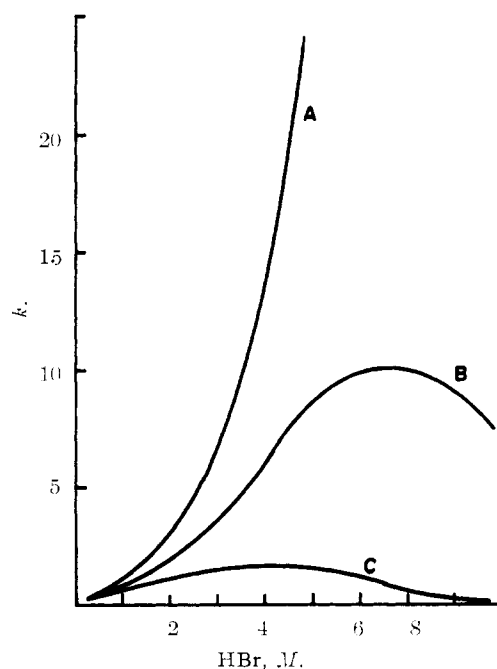
Fig. 5.—Plot of observed and calculated rate constants vs. molarity \text{HBr} : (A) 0.542 h_0 [\text{S}]/[\text{S}]_{\text{stoich}} ; (B) k_{\text{obsd}} \times 10^3 \text{ sec.}^{-1} (80^\circ) ; (C) 0.542 M [\text{S}]/[\text{S}]_{\text{stoich}} .
