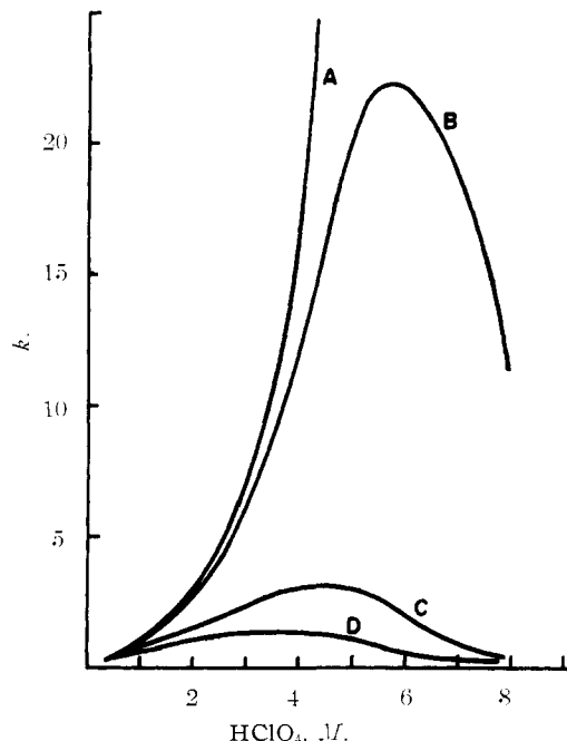
Fig. 3.—Plot of observed and calculated rate constants vs. molarity \text{HClO}_4 : (A) 0.452 k_0 [\text{S}]/[\text{S}]_{\text{stoich}} ; (B) 57.4 a_{\text{H}_2\text{O}} [\text{SH}^+]/[\text{S}]_{\text{stoich}} ; (C) k_{\text{obsd}} \times 10^3 \text{ sec.}^{-1} (80^\circ) ; (D) 0.505 M [\text{S}]/[\text{S}]_{\text{stoich}} . The proportionality constants are chosen so as to give intersection of all curves at 0.103 M \text{HClO}_4 .
