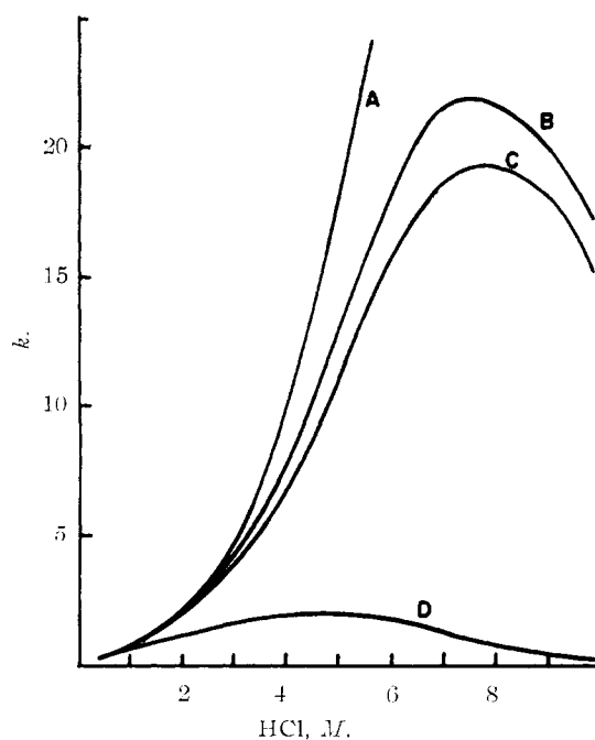
Fig. 4.—Plot of observed and calculated rate constants vs. molarity \text{HCl} : (A) 0.457 h_0 [\text{S}]/[\text{S}]_{\text{stoich}} ; (B) 58.9 a_{\text{H}_2\text{O}} [\text{SH}^+]/[\text{S}]_{\text{stoich}} ; (C) k_{\text{obsd}} \times 10^3 \text{ sec.}^{-1} (80^\circ) ; (D) 0.583 M [\text{S}]/[\text{S}]_{\text{stoich}} .
